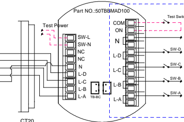
CT20 EXPLOSION CONNECTION
